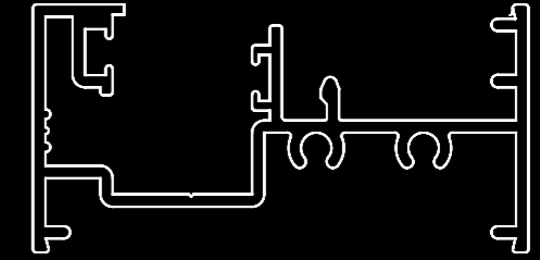
QRK-401 Glazing Frame
