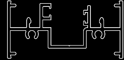
QRK-301 Glazing Frame
